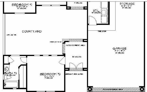
PARTIAL FLOORPLAN ELEVATION B
