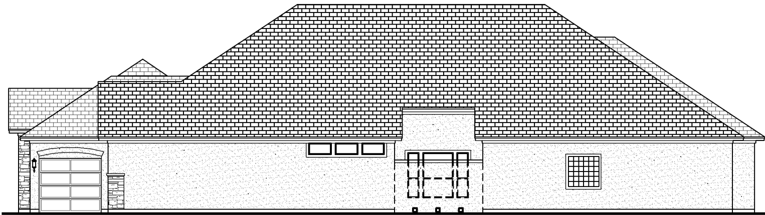
TURNBERRY II - (right elevation)
